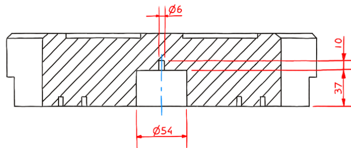
SECTIONAL END
