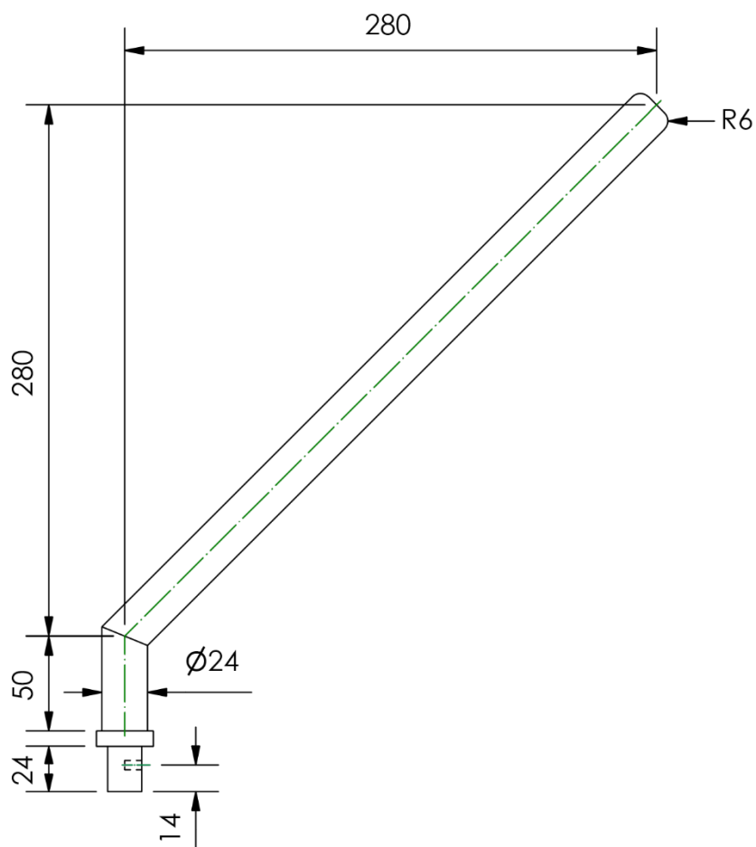
ORTHOGRAPHIC VIEW
