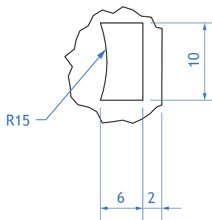
ENLARGED VIEW C
